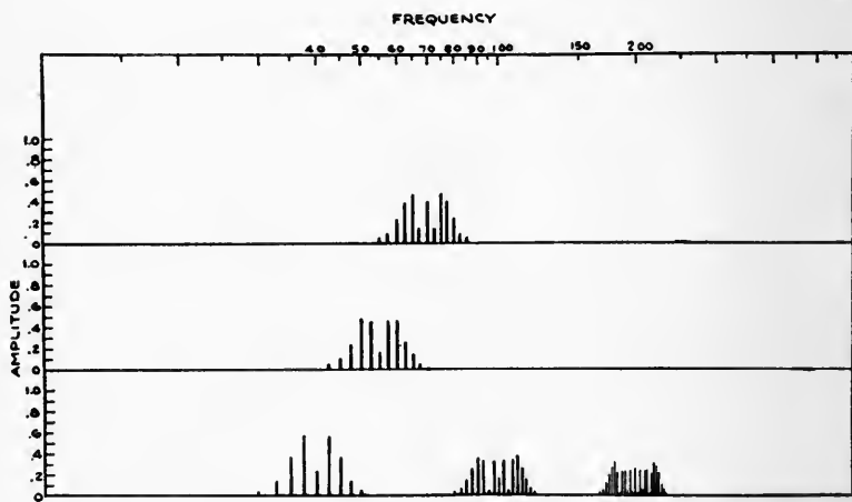
FIG. 4. Spectral distribution of warble signals: modulation \approx 12.5\% ; rate 2.5 cps; modulation sinusoidal.
